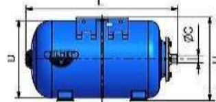
HORIZONTAL MODEL 19-24L
