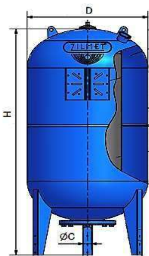
VERTICAL MODEL 50÷500L
